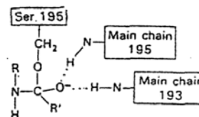
The tetrahedral transition state in the acylation reaction of chymotrypsin. The hydrogen bonds formed by two NH groups from the main chain of the enzyme are critical in stabilizing this species. This site is called the oxyanion hole .
