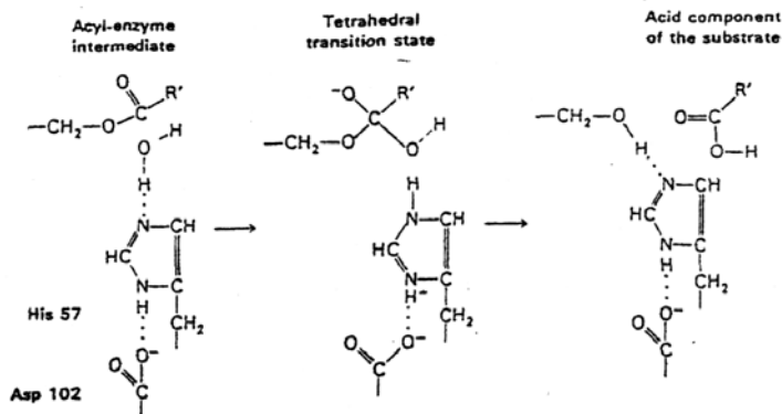
Second stage in the hydrolysis of a peptide by chymotrypsin: deacylation . The acyl-enzyme intermediate is hydrolyzed by water. Note that deacylation is essentially the reverse of acylation, with water in the role of the amine component of the original substrate.
